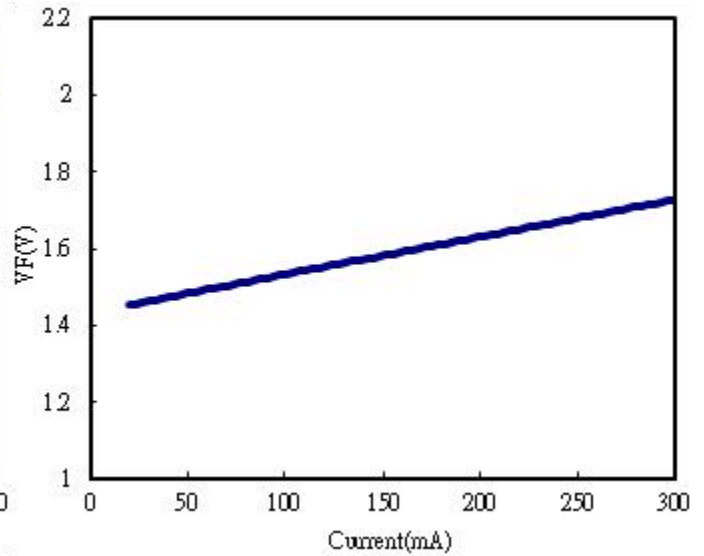
Fig.4 The V-I characteristics (0-300mA)
