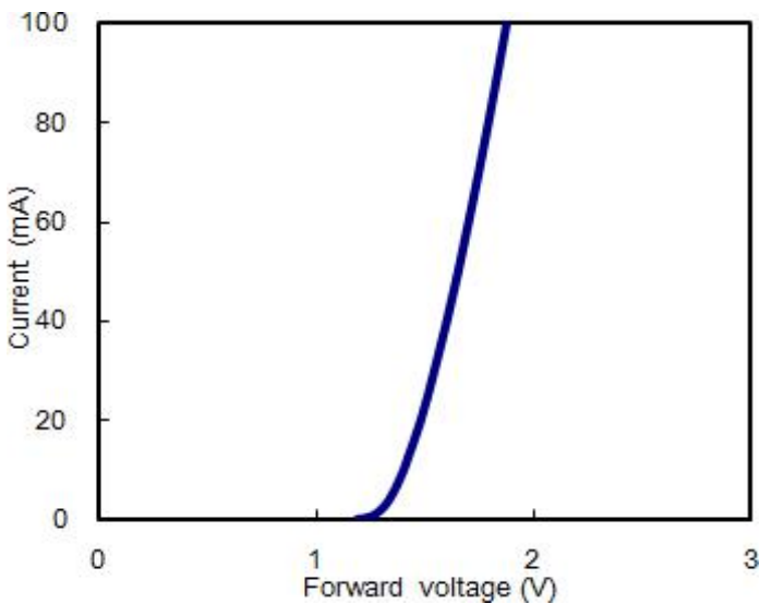
Fig.1 The I-V characteristics (0-100mA)
