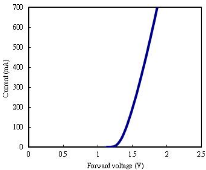
Fig.1 The I-V characteristics (0-700mA)
